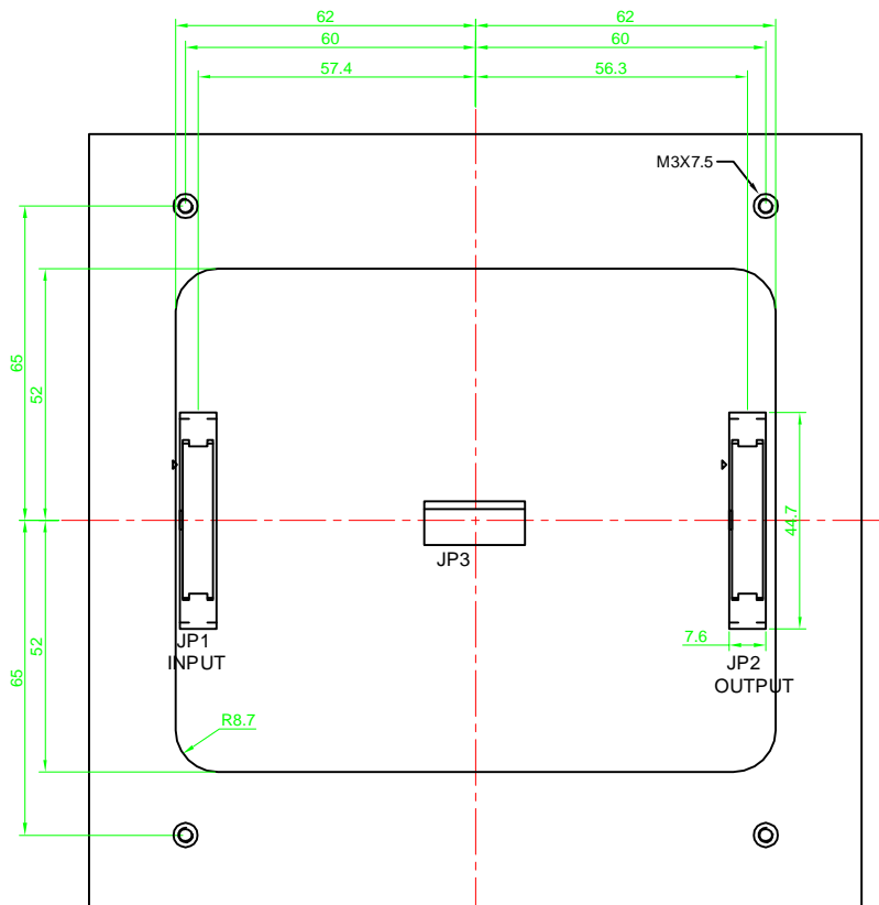
BACK VIEW
