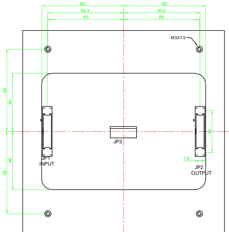
BACK VIEW
