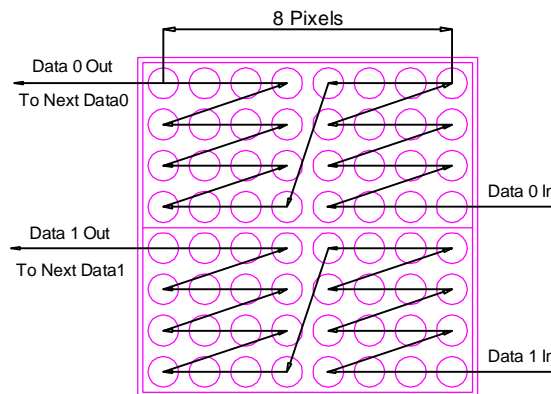
FRONT VIEW (LAMP VIEW)
